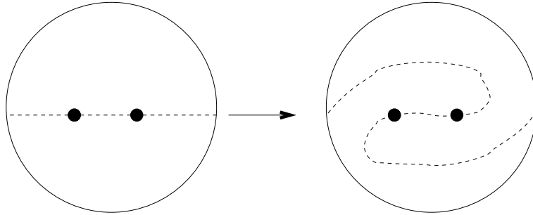
FIGURE 2. Half-twist of a two pointed disk.
